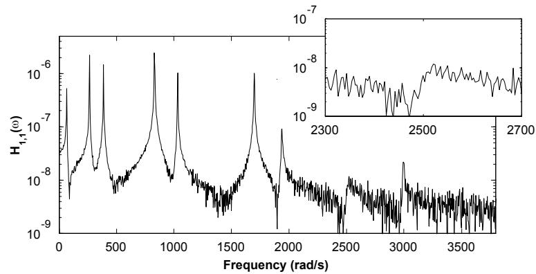
Figure 16: MIMO frame data: Noisy displacement FRF at 1 m from clamped support on beam 1.
