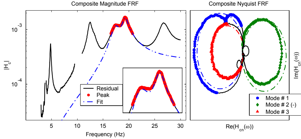
Figure 51: AMI Subtraction Step #3c (three mode fit) for Z24 data. LEFT: Composite Magnitude plots of the residual FRF data (solid) with the peak data highlighted (red dots) and the MDOF fit to the peak (dash-dot). RIGHT: Composite Nyquist plots of the isolation residual (solid) and reconstructed FRF (dash-dot) for each mode.
