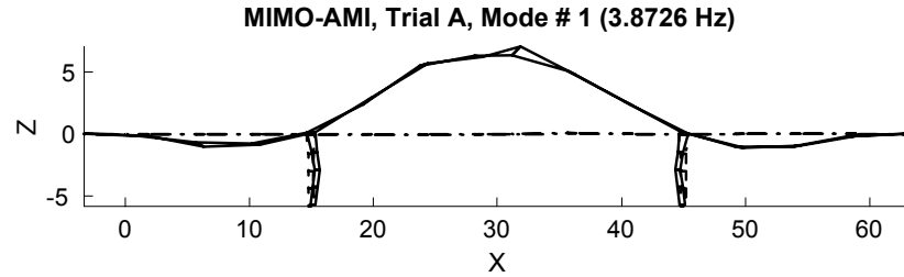
Figure 58: MIMO-AMI mode shape of Mode 1.
