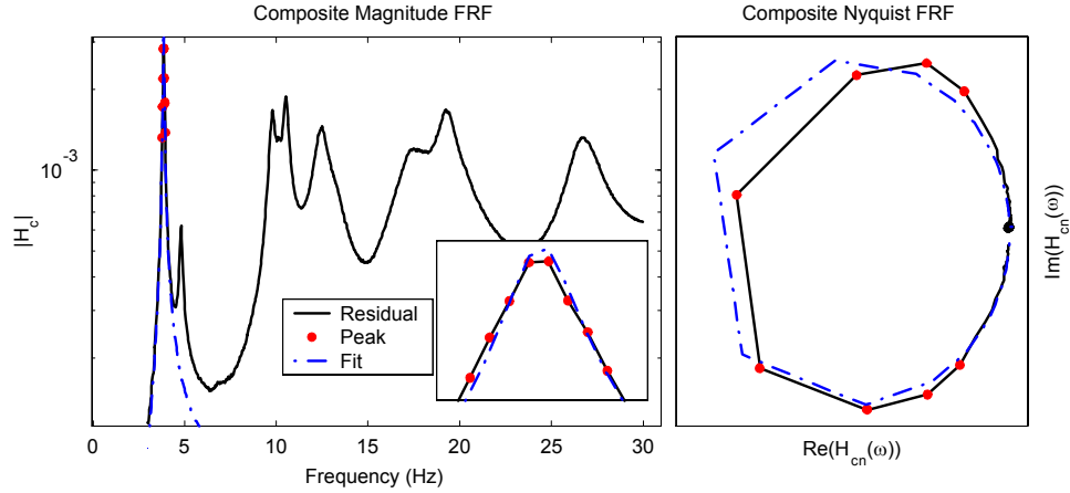
Figure 45: AMI Subtraction Step #1 (single mode fit) for Z24 data. LEFT: Composite Magnitude plots of the residual FRF data (solid) with the peak data highlighted (red dots) and the SDOF fit to the peak (dash-dot). RIGHT: Composite Nyquist plots of the residual (solid) and fit (dash-dot).
