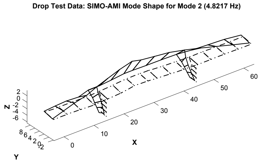
Figure 38: SIMO-AMI mode shape of Mode 2.
