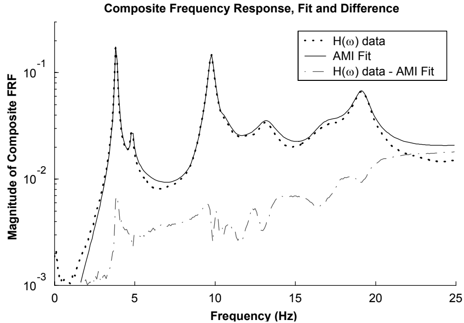
Figure 36: AMI results for Z24 bridge. Composite magnitude FRFs of data (.), AMI reconstruction (-) and the difference (-.).
