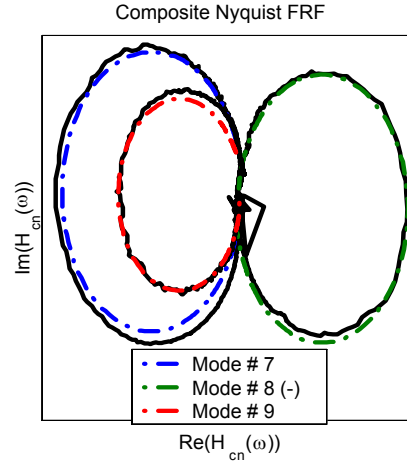
Figure 55: Composite Nyquist plots of the isolated FRFs and the reconstructed FRFs for modes 7, 8 and 9 after mode isolation and refinement.
