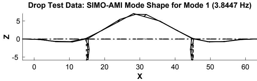
Figure 37: SIMO-AMI mode shape of Mode 1.
