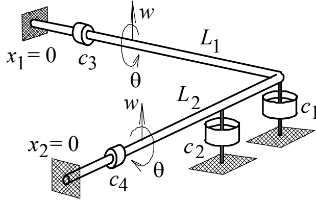
Figure 5: Schematic of Cantilevered Frame System.
